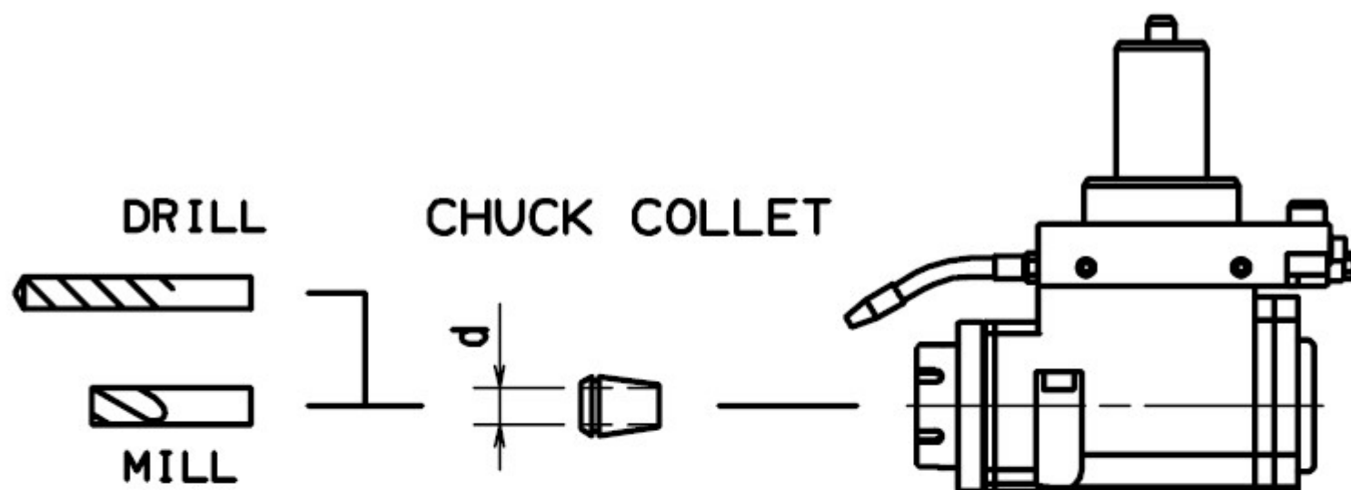
H-TYPE MILLING HOLDER (WITH \phi 20 CHUCK COLLET)
