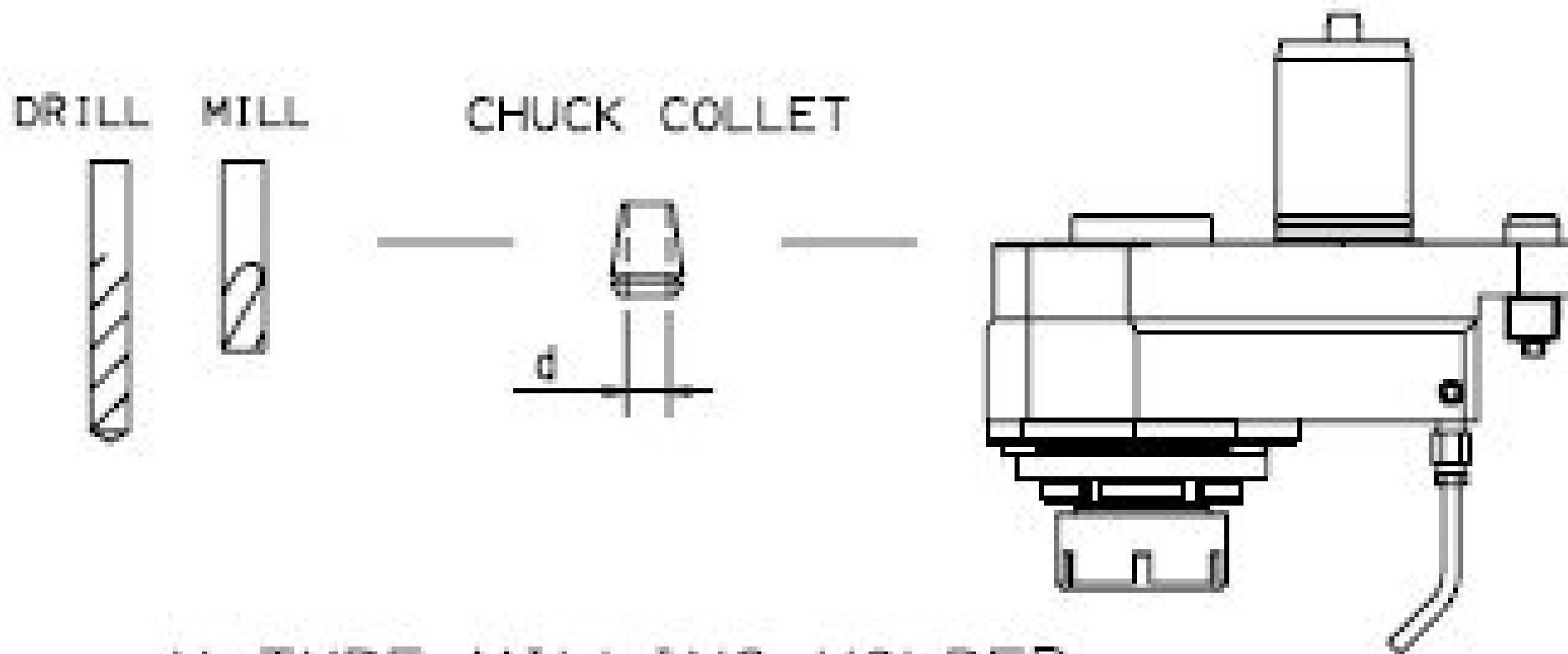
V-TYPE MILLING HOLDER (WITH \phi 25 CHUCK COLLET)
