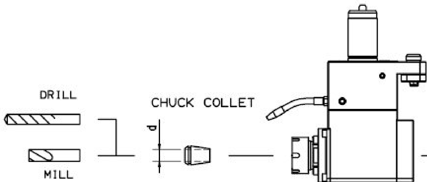
H-TYPE HD MILLING HOLDER (WITH \phi 20 CHUCK COLLET)
